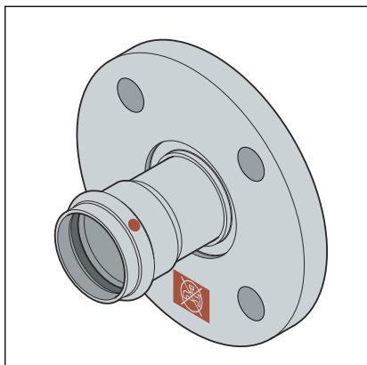
Fig. 11: Fixed flange
